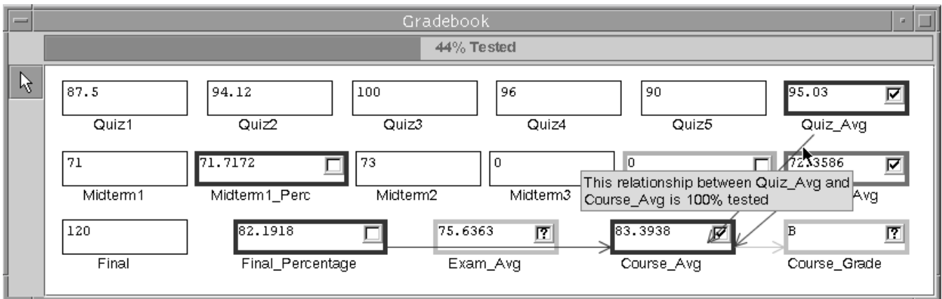
Figure 1: An example of WYSIWYT in Forms/3.
